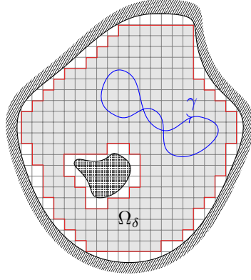
Sketch of the proof for the homological version of Cauchy's theorem .
